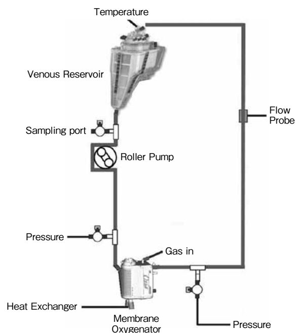
Fig. 1 Experimental recirculation circuit
